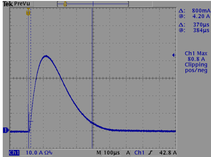
LUR-040S105ST(Io=700mA)
