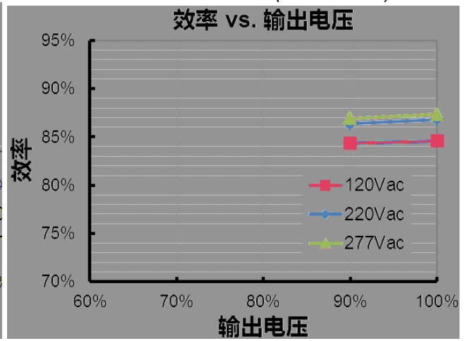
LUR-040S150ST (Io=1500mA)
